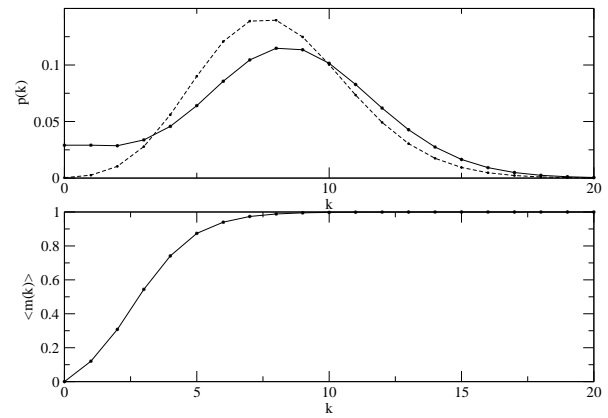
FIG. 4: Results from the analytic solution. Upper plot: Plot of the degree distribution, p(k) for \eta/\lambda = 4 , showing also the Poisson distribution with the same \langle k \rangle for comparison (dashed lines). Note that the degree distribution is not Poissonian. Lower plot: Plot of the average magnetisation of a node of degree k for \eta/\lambda = 4 , showing that more highly connected nodes are, on average, more magnetised. q = 10 .
