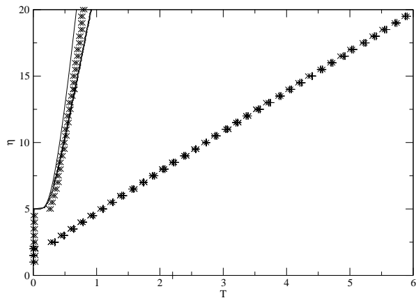
FIG. 6: Phase diagram in \eta ( \lambda = 1 ) and T , showing the high and low connectivity phases and the hysteretic region. Crosses are simulations ( n = 5000, 10000 ), plusses are theory, the points are in pairs, one on each side of the phase line. The curves are theory, the leftmost curve is \eta_c = (q/2)(\exp(1/T) + q - 1)/(\exp(1/T) - 1) which is the expected transition line if the system gets stuck in the metastable, unmagnetised state. The right curve is found using the normal method described above.
